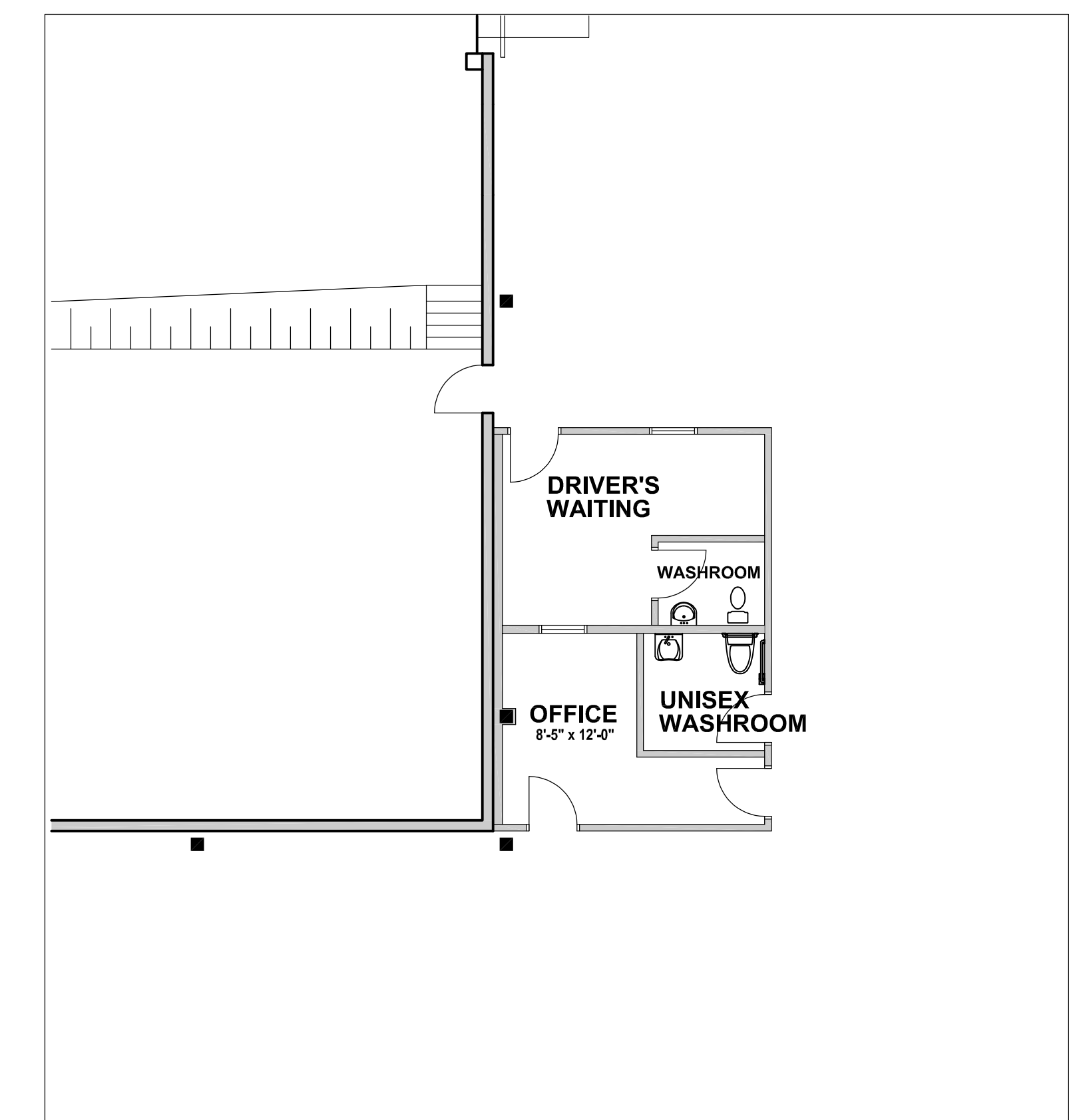
DRIVER WAITING ROOM AND DISPATCH OFFICE SCALE: 1/8" = 1'-0" WHEN PRINTED ON 24" x 36" SHEET SCALE: 0 5 10 20 FEET
